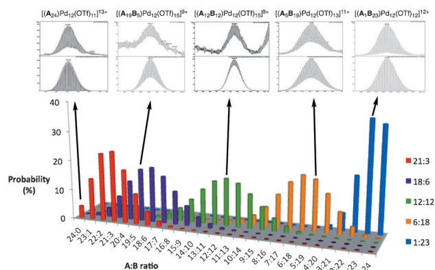
Figure 4. Top: Illustrative peaks in the CSI-MS spectra [measured (top) spectrum versus simulated spectrum (bottom)] of selected spheres ( \mathbf{A}_n\mathbf{B}_{24-n}\text{Pd}_{12}(\text{OTf})_{24} ) present in the statistical mixture. Bottom: Binomial distribution of spheres ( \mathbf{A}_n\mathbf{B}_{24-n}\text{Pd}_{12}(\text{OTf})_{24} ) formed at different \mathbf{A}/\mathbf{B} ratios: 1:23 (blue), 6:18 (orange), 12:12 (green), 18:6 (violet), 21:3 (red) with a palladium(II) precursor.
